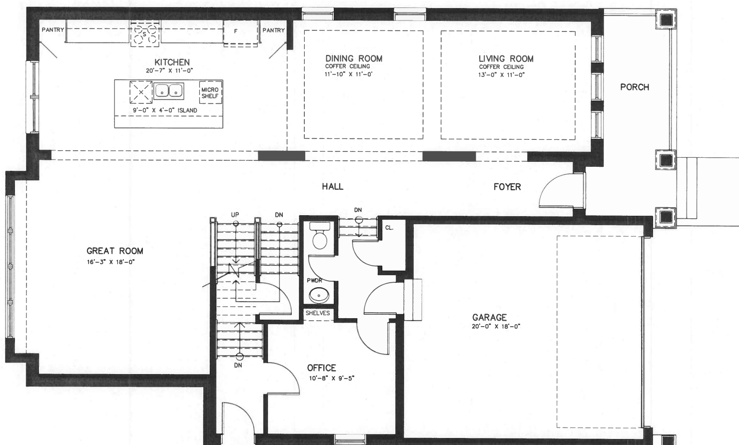
FIRST FLOOR PLAN 1400 SQUARE FEET
