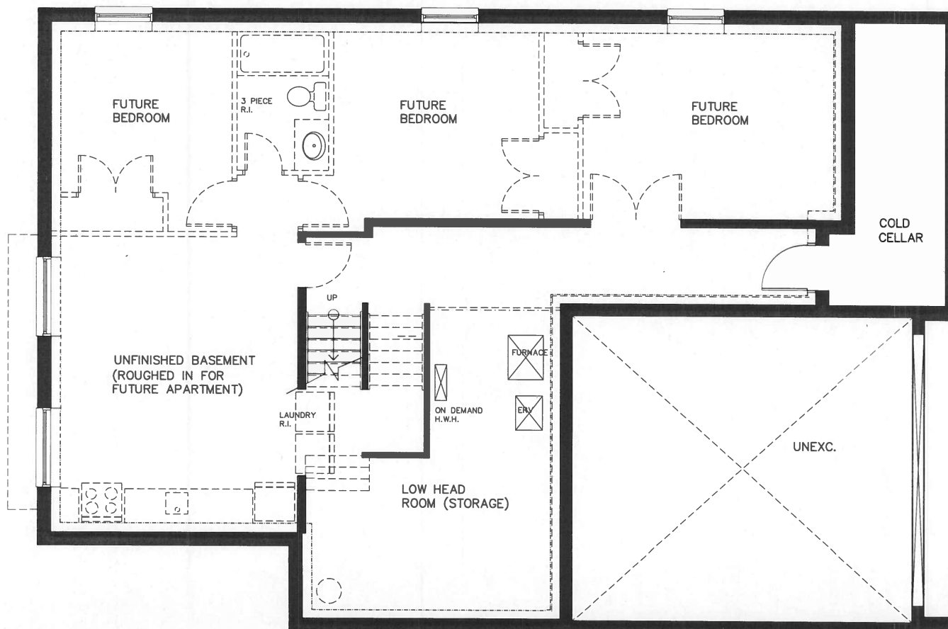
BASEMENT PLAN
