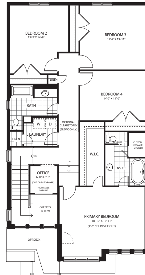
SECOND FLOOR (4 BED OPT.) 1729 SQ.FT. (INCLUDES OPEN TO BELOW)
