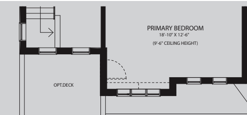
SECOND FLOOR (4 BED) 1694 SQ.FT. (INCLUDES OPEN TO BELOW)
