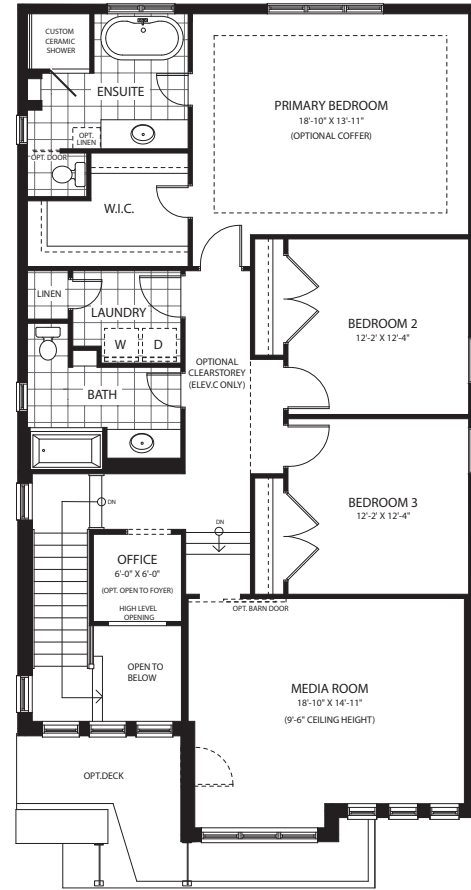
SECOND FLOOR (MEDIA ROOM OPT.) 1729 SQ.FT. (INCLUDES OPEN TO BELOW)
