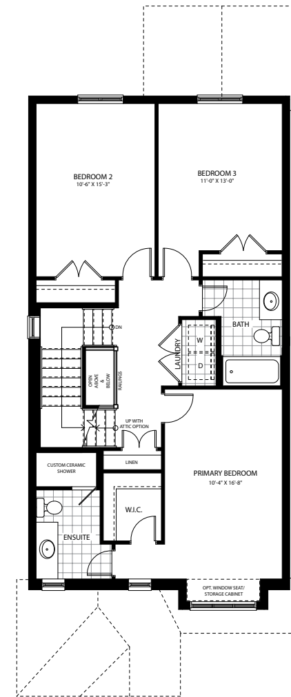
SECOND FLOOR 1014 SQ.FT. (INCLUDES OPEN TO BELOW)
