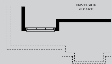
OPTIONAL ATTIC FLOOR - 707 SQ.FT. (INCLUDES OPEN TO BELOW)
