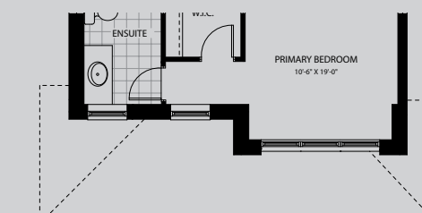
SECOND FLOOR 1026 SQ.FT. (INCLUDES OPEN TO BELOW)
