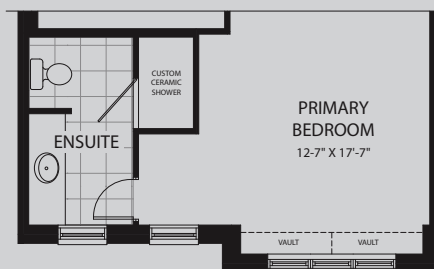
SECOND FLOOR - 1062 SQ.FT. (INCLUDES OPEN TO ABOVE WITH OPT. ATTIC)
