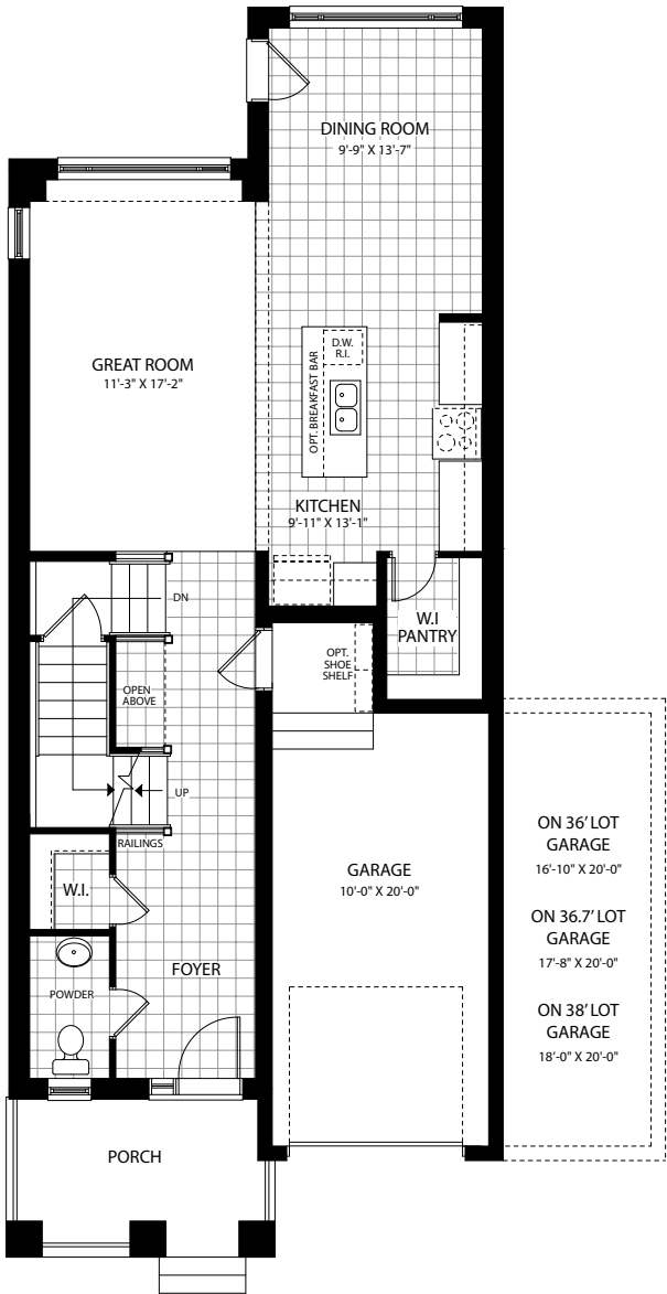
MAIN FLOOR 865 SQ.FT.
