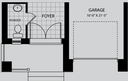
MAIN FLOOR 864 SQ.FT.
