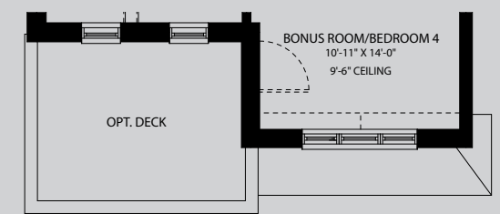
SECOND FLOOR 1244 SQ.FT. (INCLUDES OPEN TO BELOW)
