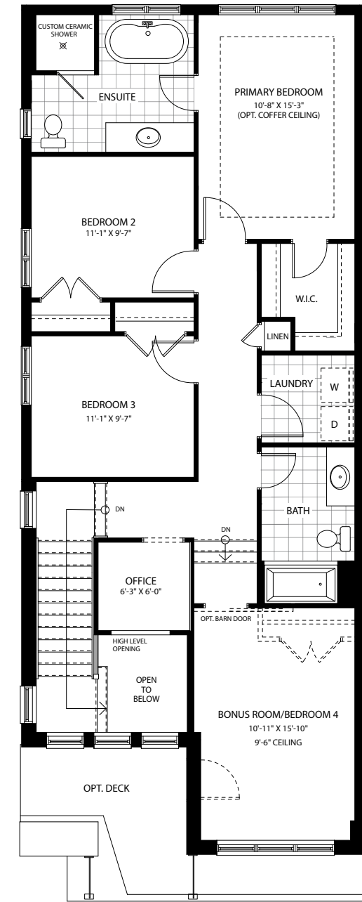
SECOND FLOOR - 1264 SQ.FT. (INCLUDES OPEN TO BELOW)
