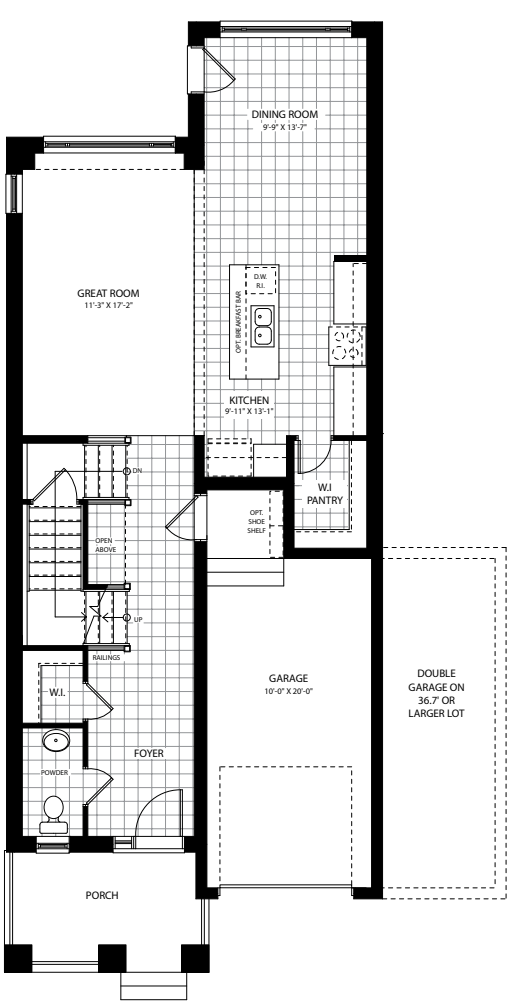
MAIN FLOOR 865 SQ.FT.
