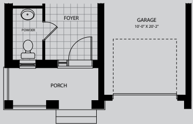
MAIN FLOOR 852 SQ.FT.
