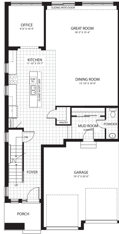
MAIN FLOOR 1208 SQ.FT.
