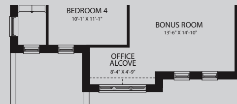
SECOND FLOOR - 1598 SQ.FT.
