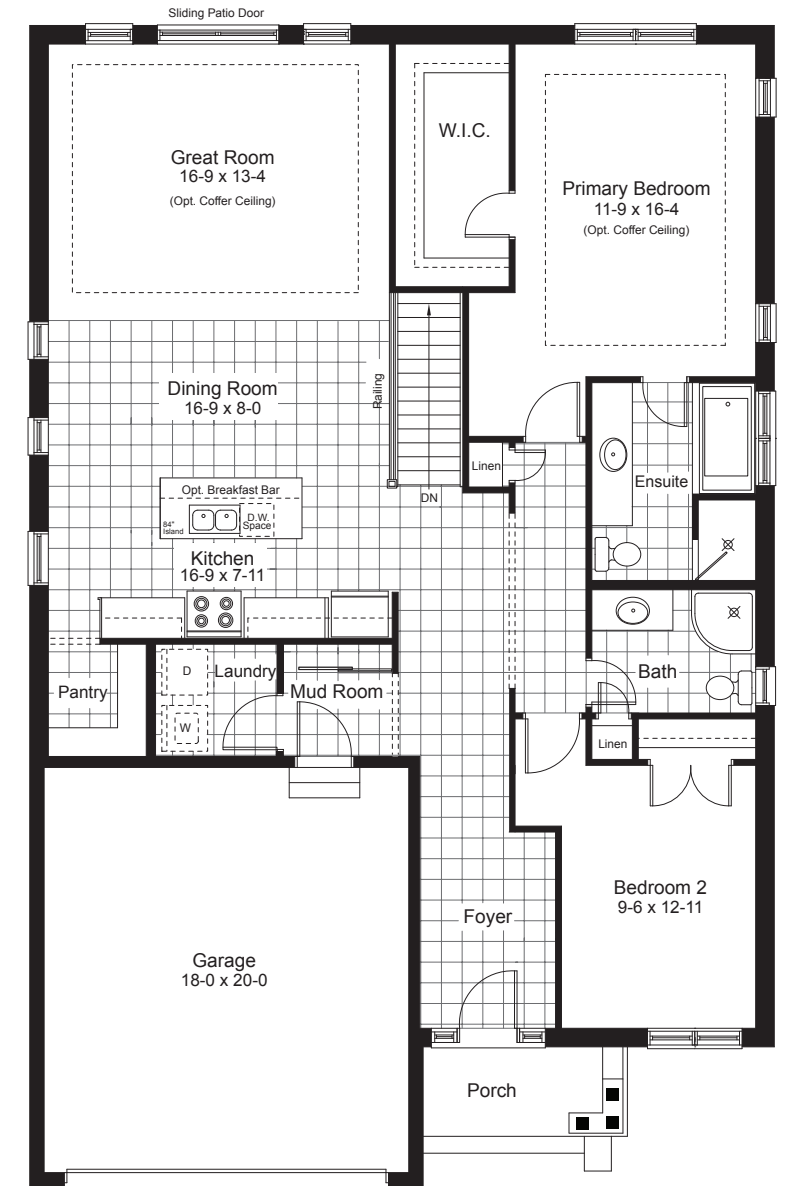
ALTERNATE MAIN FLOOR 1594 SQ.FT.
