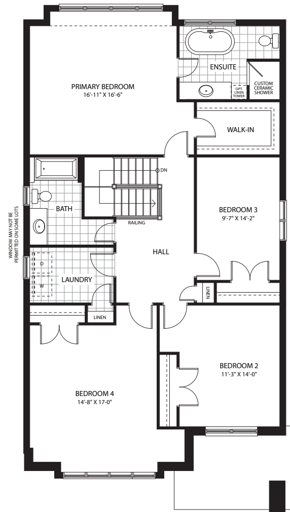
SECOND FLOOR (4 BED OPT. WITH MAIN FLOOR OFFICE) 1550 SQ.FT.
