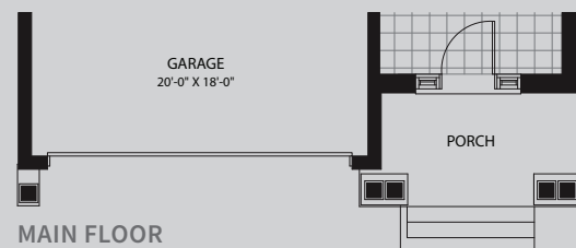
MAIN FLOOR 1140 SQ.FT.
